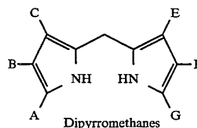
Dipyrromethanes
