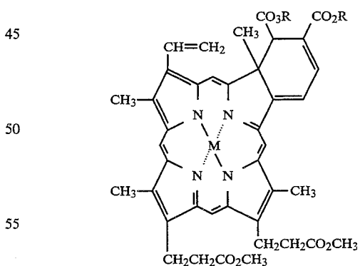
Complex VIII
