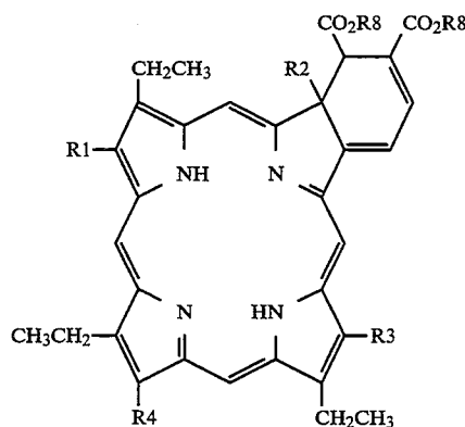
Formula 2
