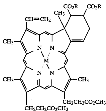
Complex X
