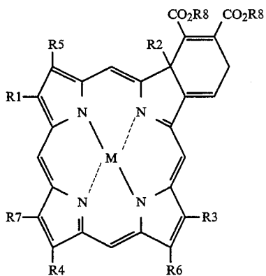
Formula 3
