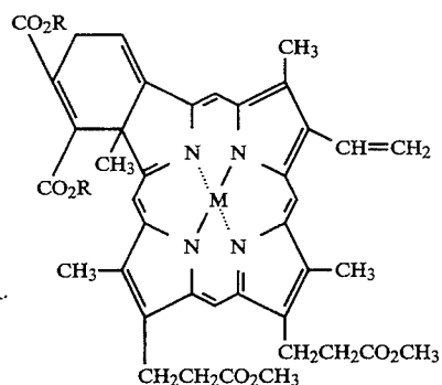
Complex V
