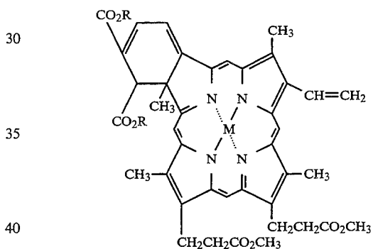
Complex VII
