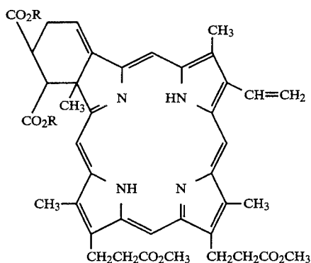
Adduct IX
