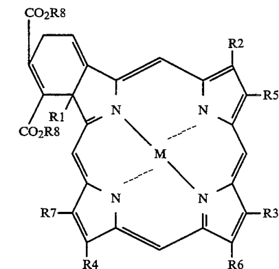
Formula 2
