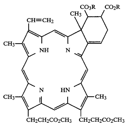
Adduct X
