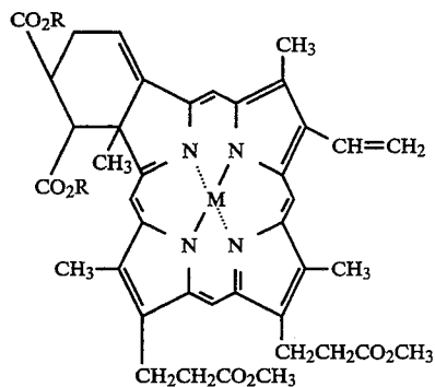
Complex IX
