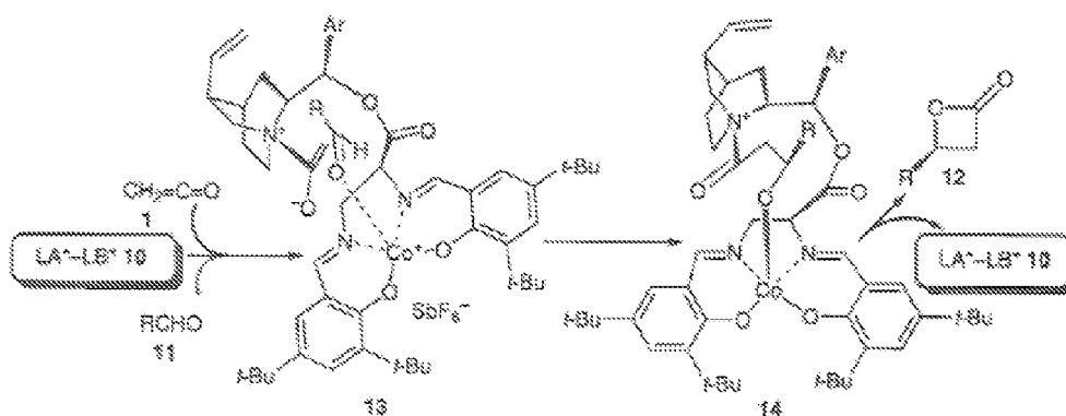
FIGURE 5 - Scheme 5
