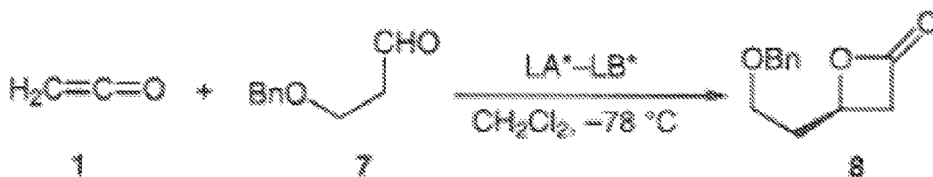
FIGURE 2 - Scheme 2
