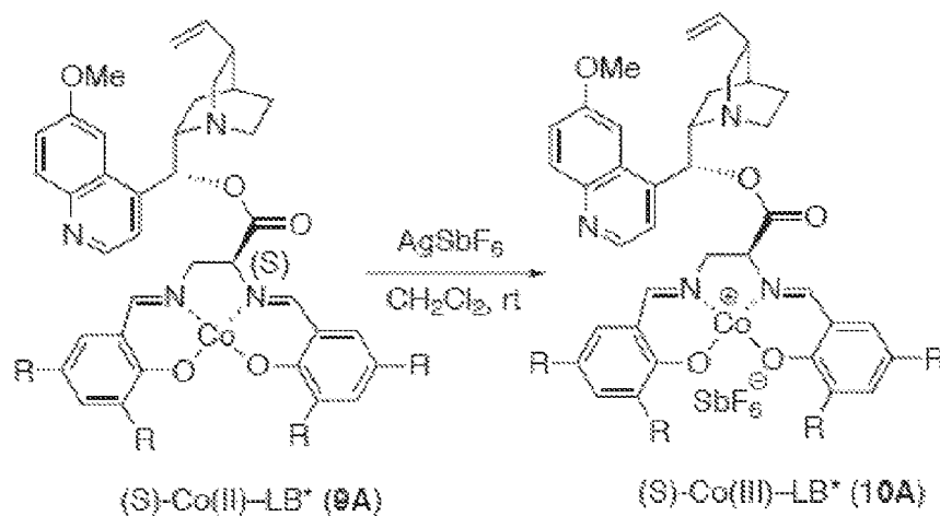
FIGURE 7 - Scheme 7
