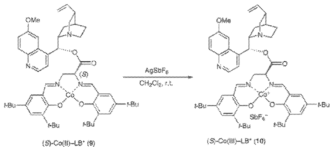
FIGURE 3B - Scheme 3
