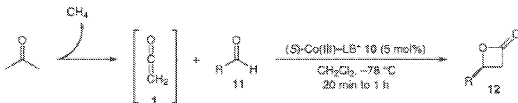
FIGURE 4 - Scheme 4
