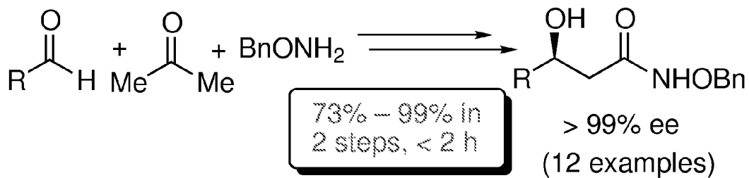
FIGURE 6 - Scheme 6
