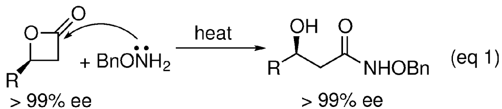
FIGURE 8 - Scheme 8
