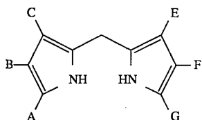
Dipyrromethanes
