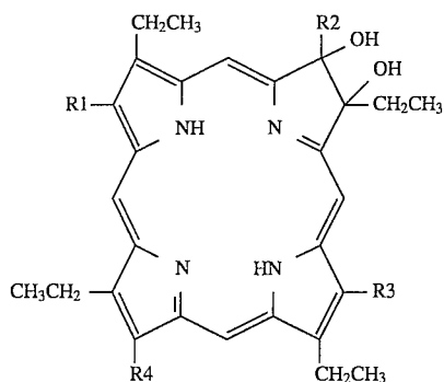
Dihydroxy Chlorins
