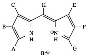
Dipyrromethenes
